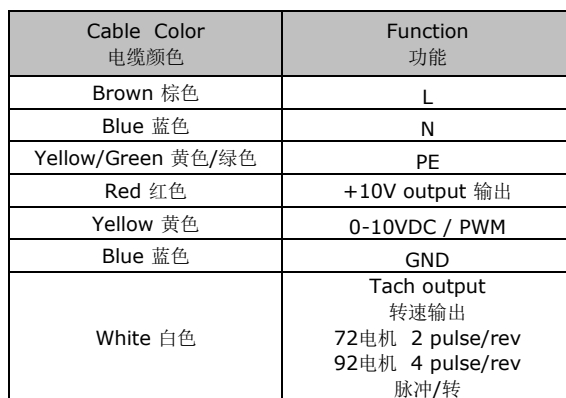
Wire Diagram
