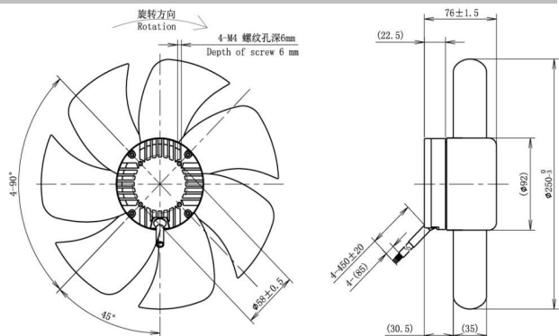
A1SE250 Without Grid 不带网罩
